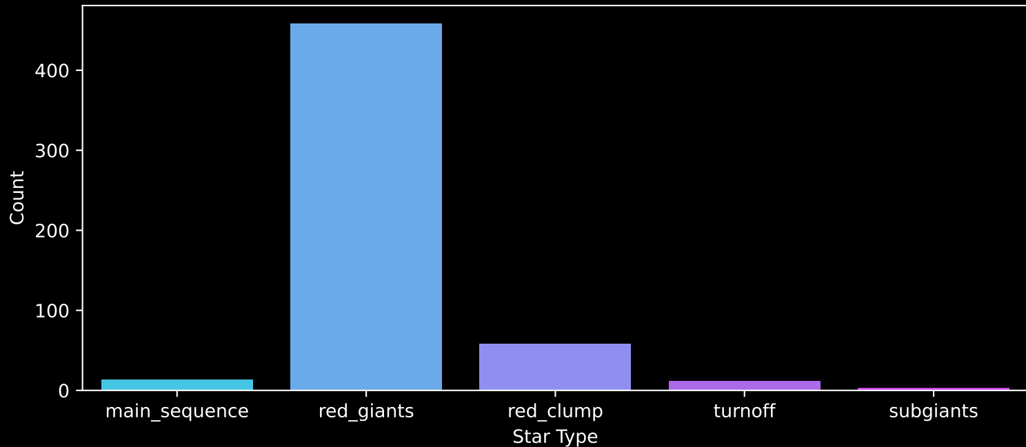
APOGEE DR17 Field: [064-06] Count plot of Star Type
