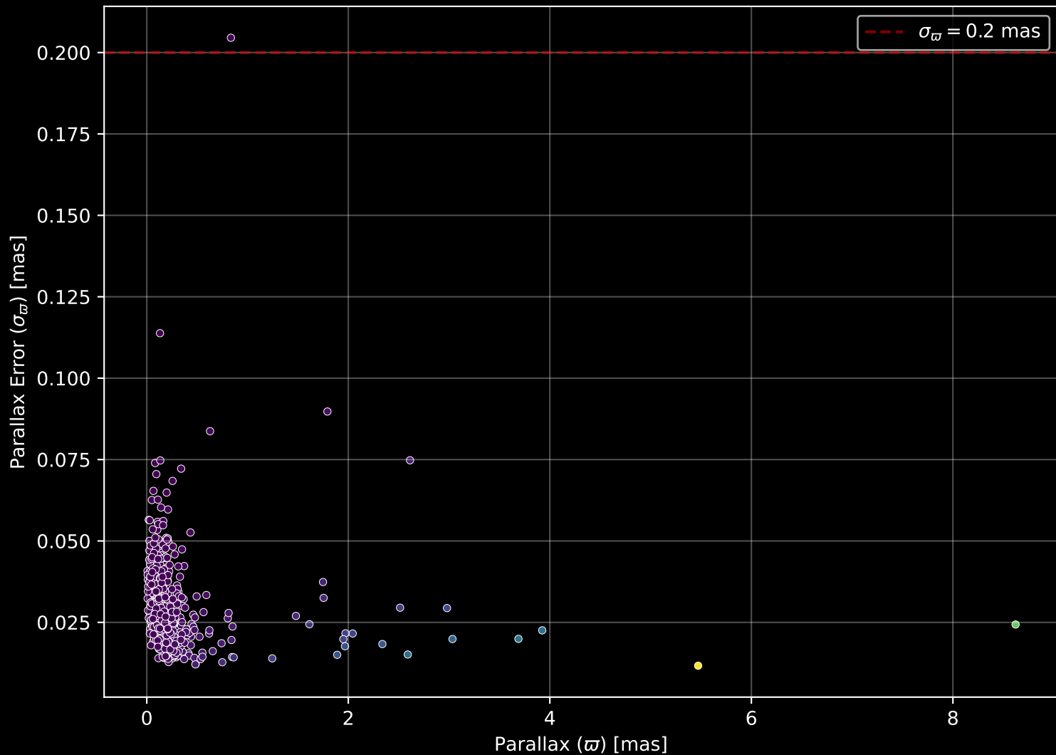
APOGEE DR17 Field: [064-06] Parallax Quality (n= 544)
