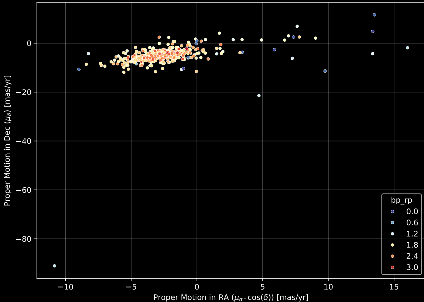
APOGEE DR17 Field: [064-06] Proper Motion Diagram (n= 544)
