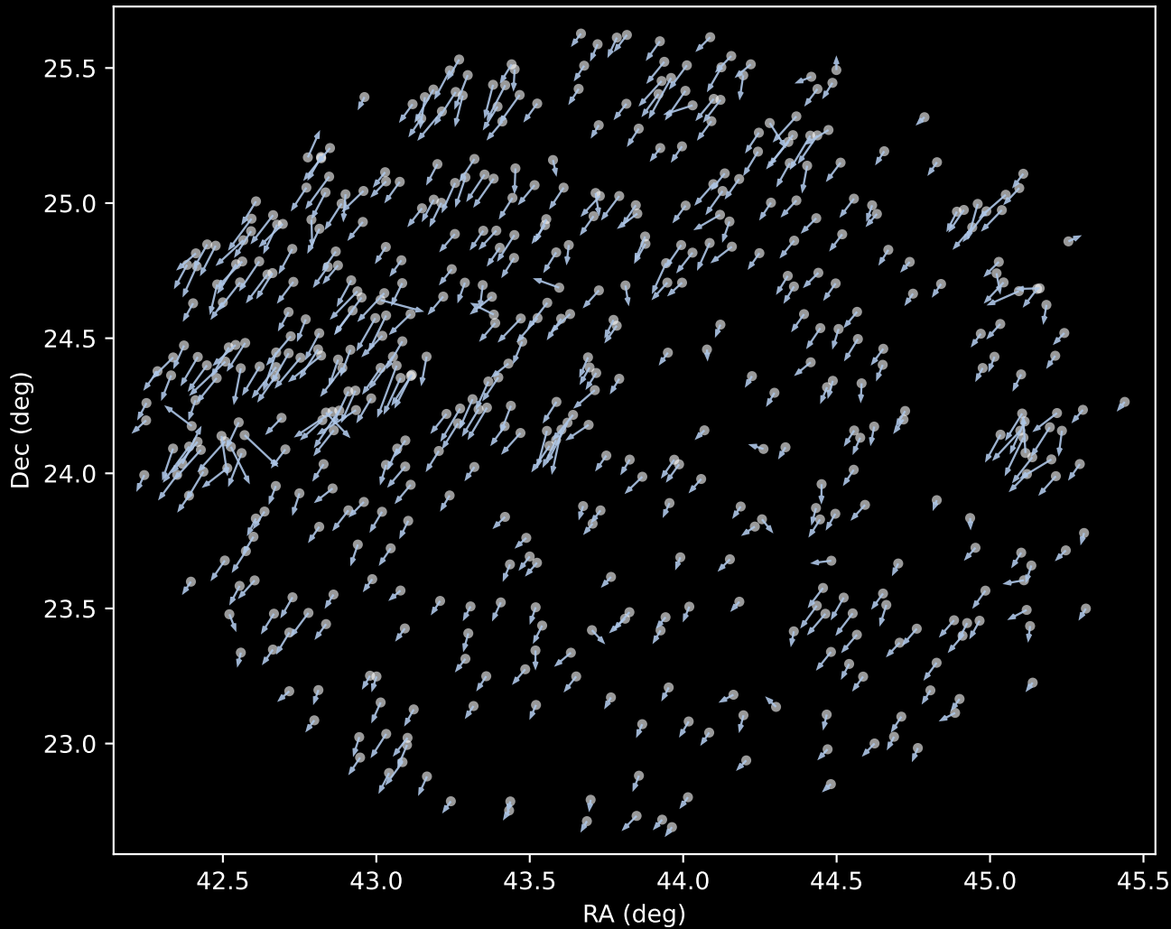
APOGEE DR17 Cluster 1 Proper Motion Vectors (n=521)
